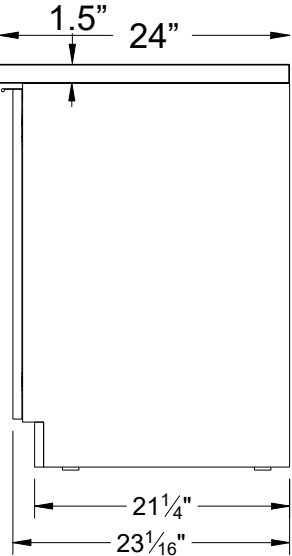
3 18 RIGHT SIDE ELEVATION
