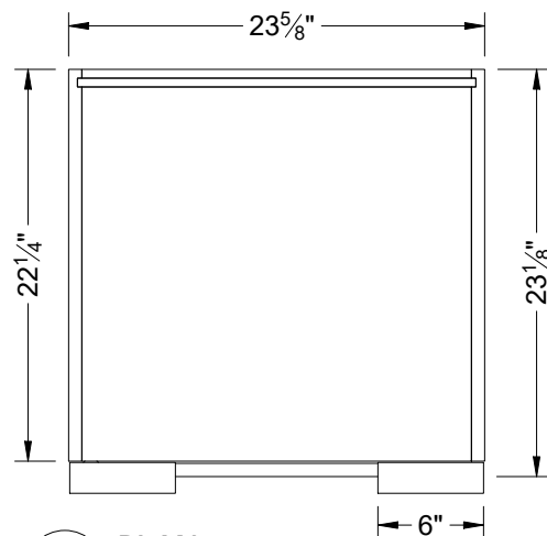
1 PLAN 2' SINGLE LEFT CABINET
