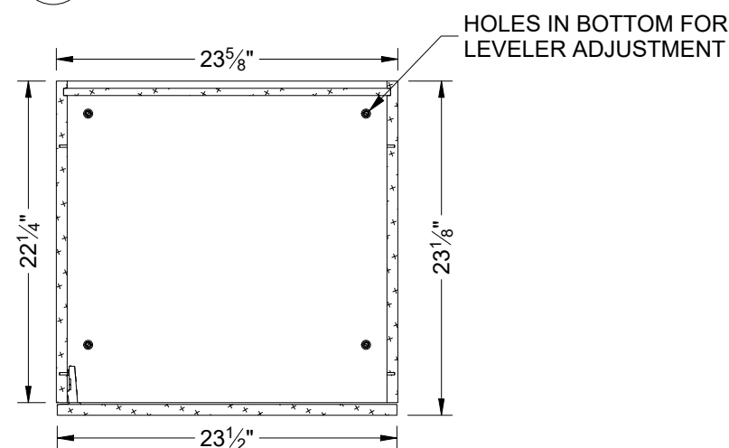
B SECTION 2' SINGLE LEFT CABINET
