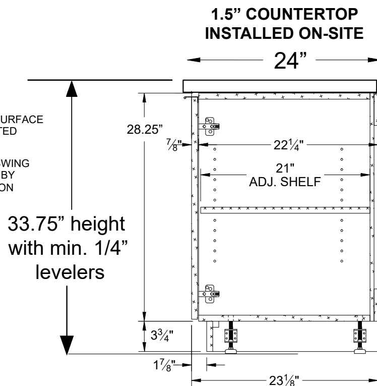
A SECTION 1"=1' 2' SINGLE LEFT CABINET
