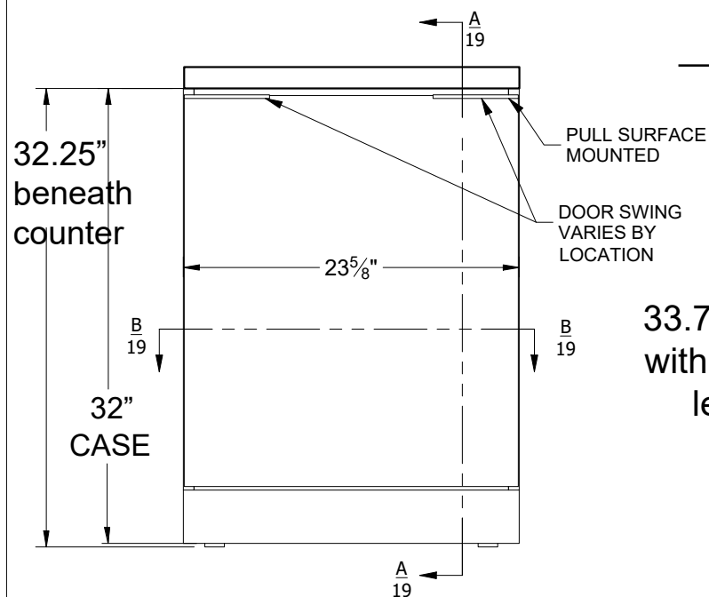
2 ELEVATION 2' SINGLE LEFT CABINET
