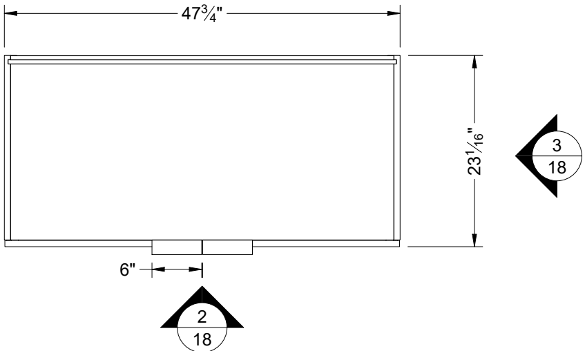
1 18 PLAN VIEW
