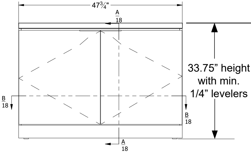
B 18 PLAN SECTION
